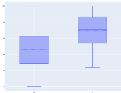
Figure 6: Boxplot
