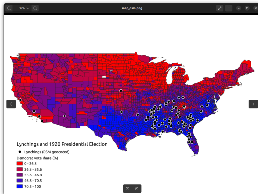
Figure 11: OSM map
